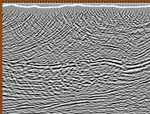
Pre-Stack Depth Migration - Initial Velocity Model
