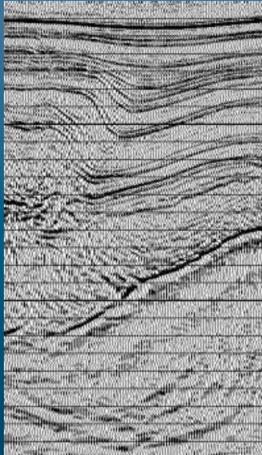
Finite-Offset Pre-Stack Time Migration
