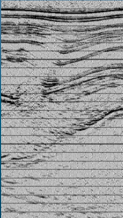
Post-Stack Phase-Shift Time Migration
