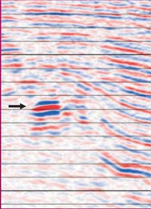
Class-3 Bright Spot
