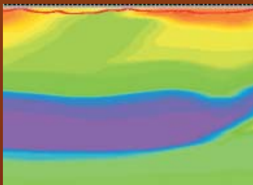
Final Velocity Model with Tomographic Inversion
