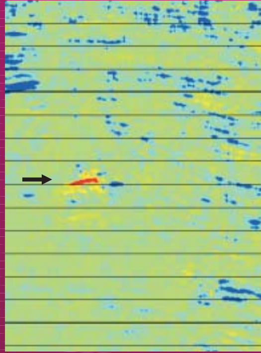
A x B Intercept Gradient
