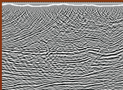
Pre-Stack Depth Migration - Final Velocity Model
